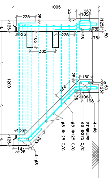
REINFORCEMENT PLAN
