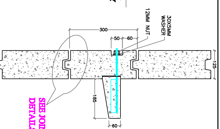
DETAILS OF FIXING FOOT STEP
